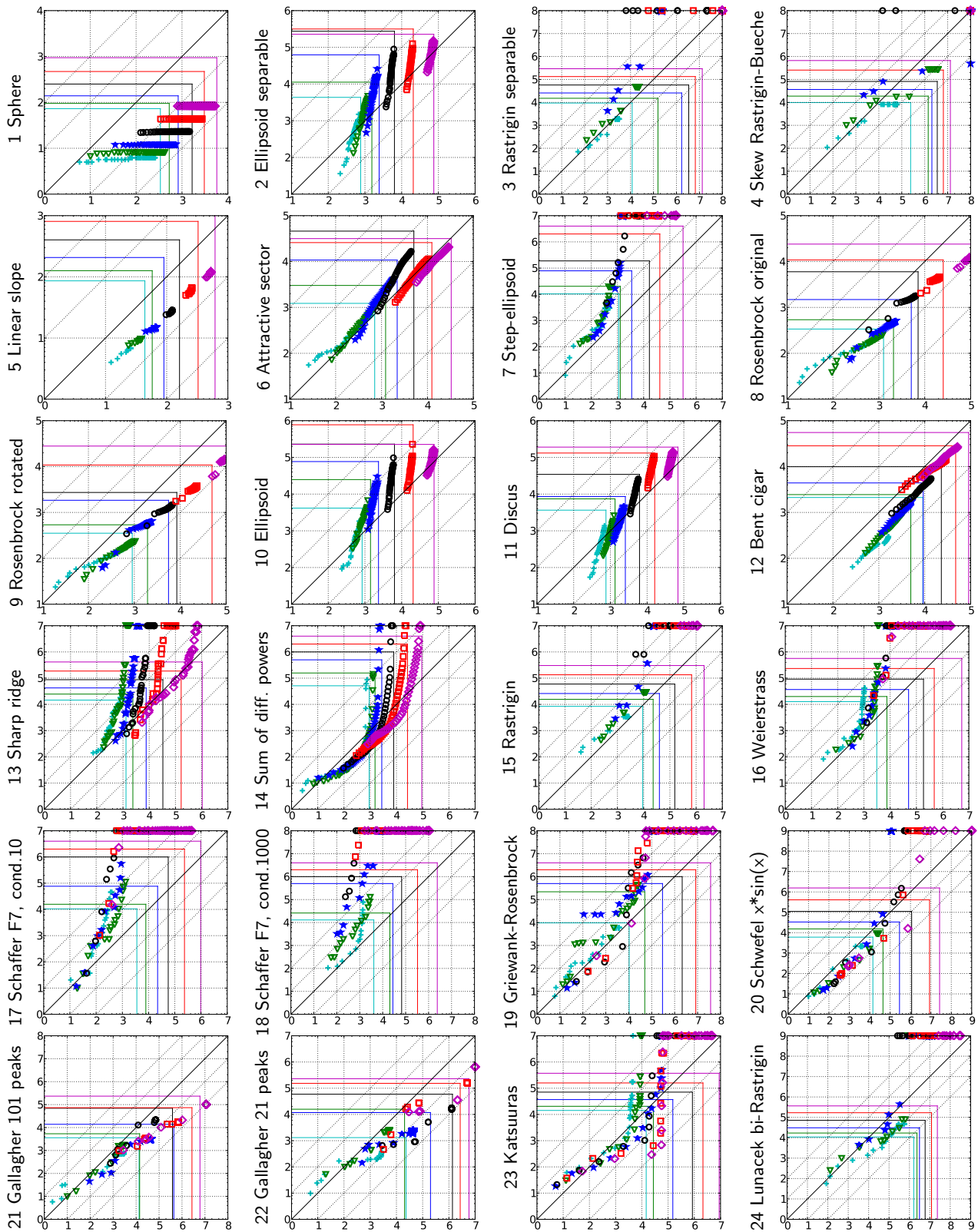
Figure 2: Expected running time (ERT in \log_{10} of number of function evaluations) of NEWUOA versus BIPOP-CMA-ES for 46 target values \Delta f \in [10^{-8}, 10] in each dimension for functions f_1-f_{24} . Markers on the upper or right edge indicate that the target value was never reached by NEWUOA or BIPOP-CMA-ES respectively. Markers represent dimension: 2:+, 3:∇, 5:*, 10:○, 20:□, 40:◇. The colored lines indicate maximum number of function evaluations
