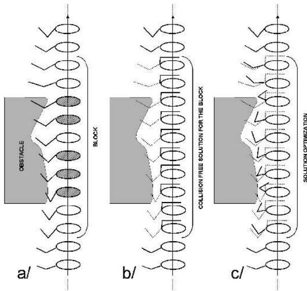
Figure 6: Warping method steps
