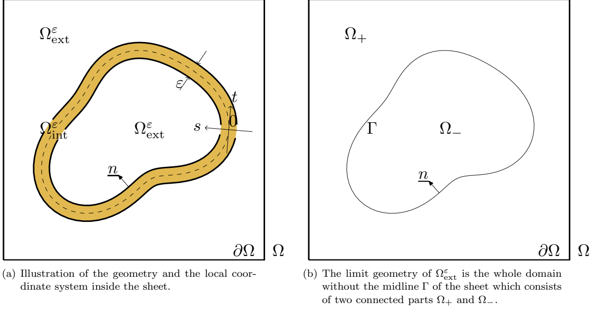
FIGURE 1. The two-dimensional geometrical setting for a sheet of thickness \epsilon and the limit geometry for \epsilon \rightarrow 0 .
