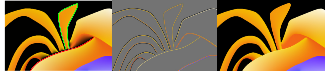
Figure 7: Left: Lines along which problems occur. Center: Red and green line curves are transformed into barrier curves emitting colors from only one of its sides. Right: Result of the diffusion.
