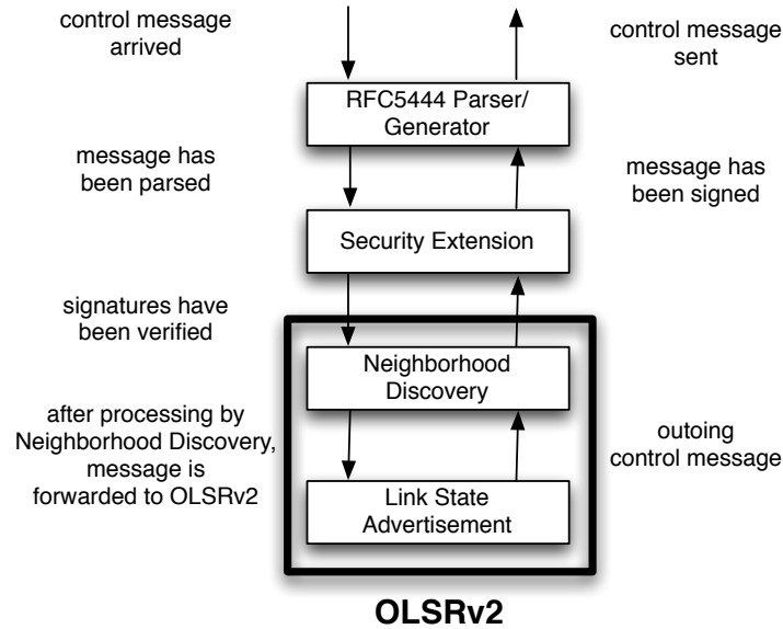
Figure 3: Message flow between NHDP, OLSRv2 and the security extension
