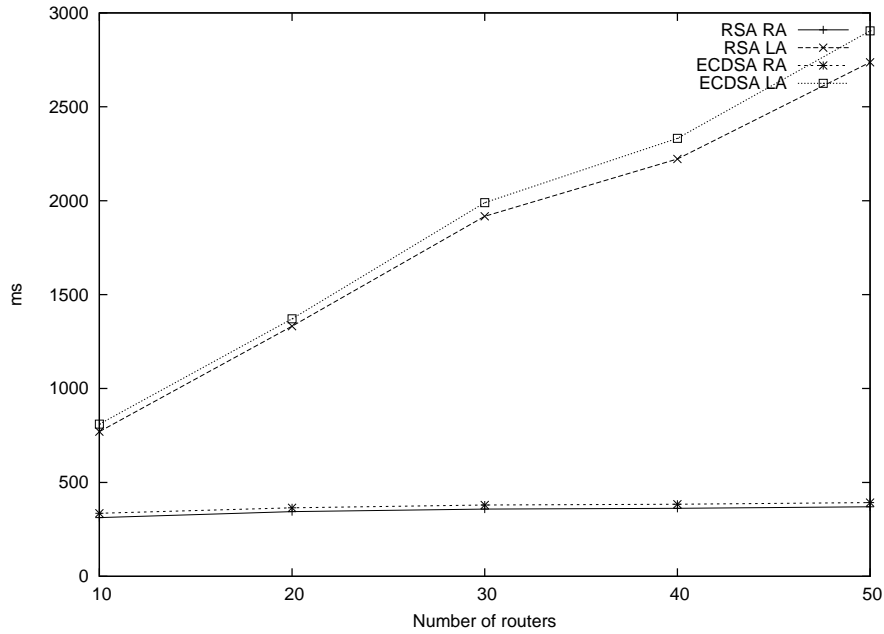
Figure 6: Cumulative time per router spent on generating message signatures.
