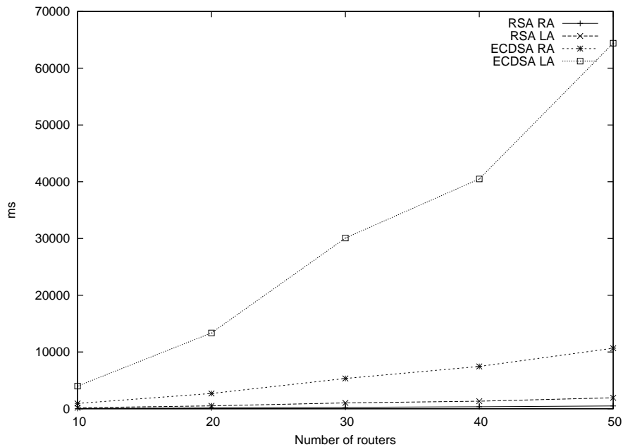
Figure 7: Cumulative time per router spent on verifying message signatures.
