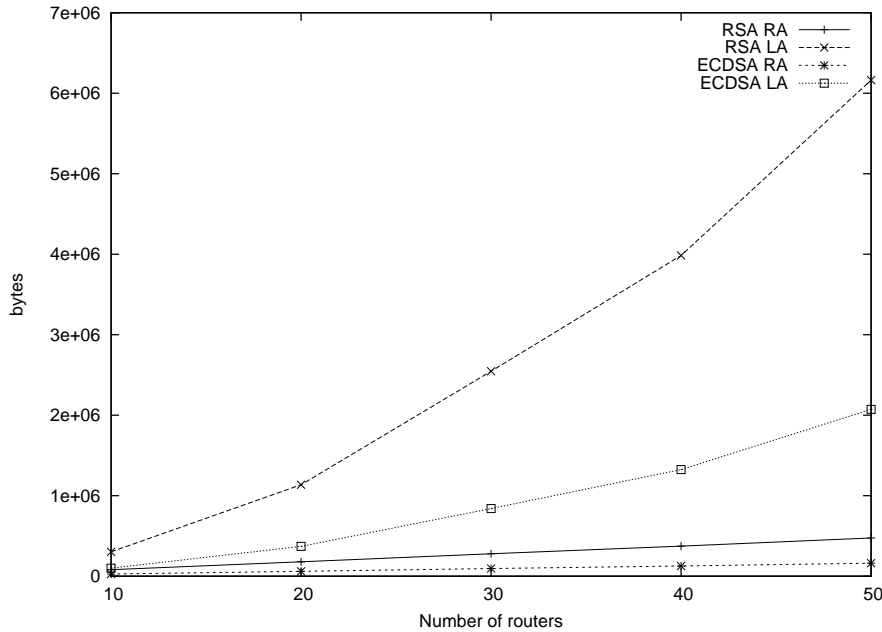
Figure 5: Total overhead incurring due to signature inclusion.
