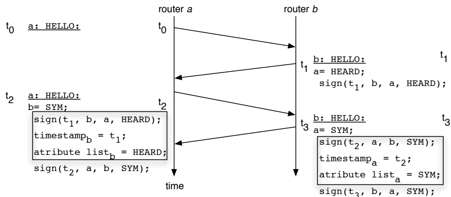
Figure 2: Example of link admittance control in the Neighborhood Discovery process of OLSRv2: attributes listed in “boxes” are those received from the “peer” in a previous HELLO message.
