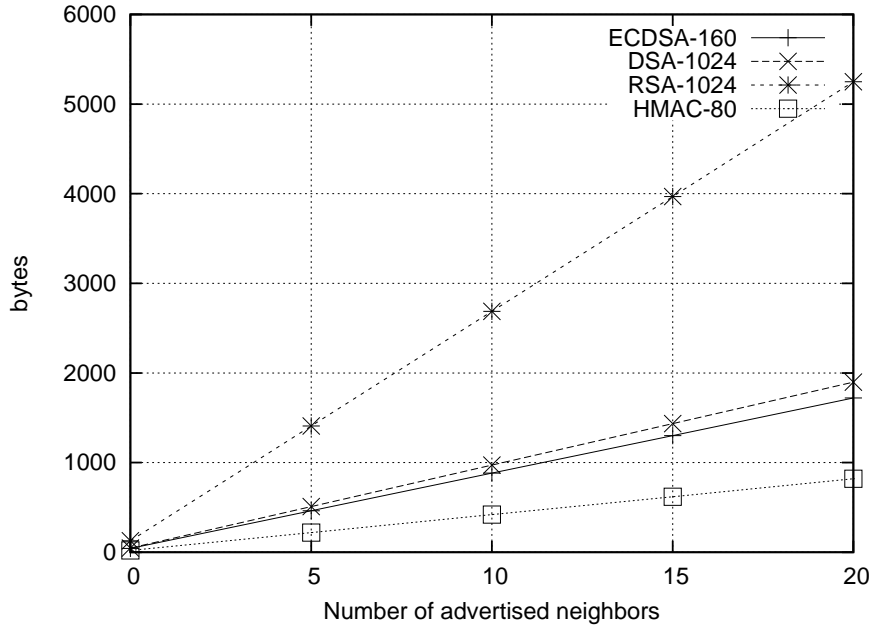
Figure 4: Link admittance control: Signature overhead per control message with increasing number of advertised neighbors
