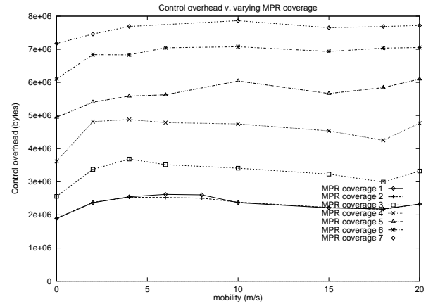
Figure 3. Control traffic overhead from ns2 simulations.
