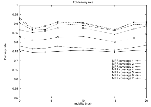
Figure 2. Delivery rate of TC-messages from ns2 simulations.
