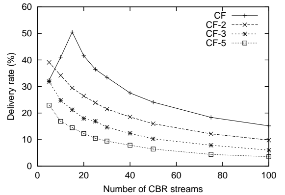
Figure 5. Multipacket Flooding: Delivery Rate of Classical Flooding
