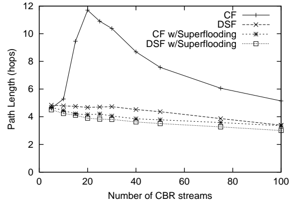
Figure 4. Path length (hops) with varying number of streams
