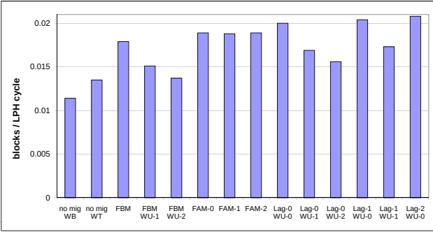
Figure 4: Arithmetic mean over all benchmarks of the shared-bus activity in blocks per LPH cycle. The two leftmost bars are for the baseline with migration disabled, with a write-back (WB) and write-through (WT) L2.
