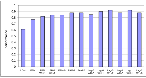
Figure 3: Harmonic mean over all benchmarks of the performance normalized to the baseline (8 GHz, no migration), assuming a fixed migration interval of 200,000 cycles (8 GHz).
