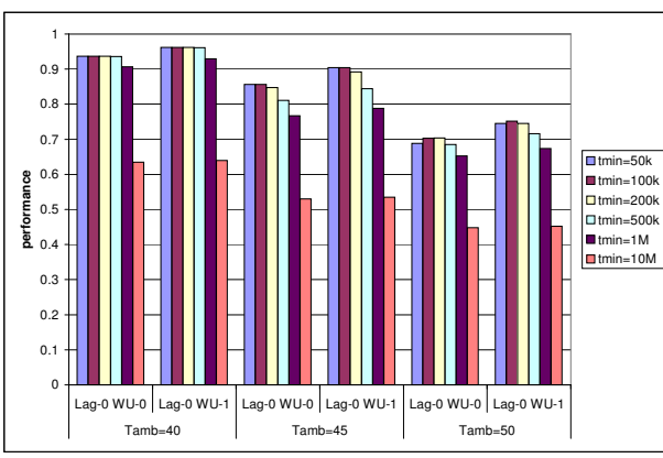
Figure 6: Harmonic mean of the normalized performance for T_{amb} = 40, 45, 50 °C and t_{min} = 50k, 100k, 200k, 500k, 1M, 10M LPH cycles.
