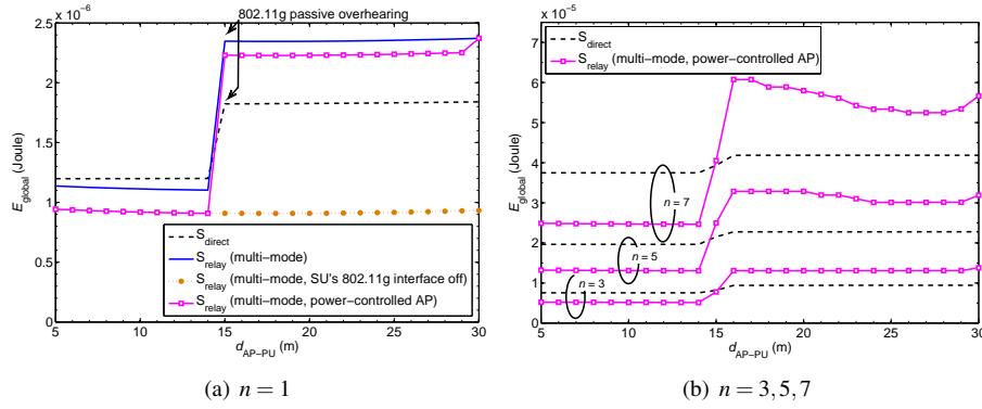
Figure 9: Comparison of energy per bit for direct or 802.15.2-to-802.11g relayed communication for n SUs, in uplink using WSN simulations, including 802.11g deactivation and power-controlled transmission
