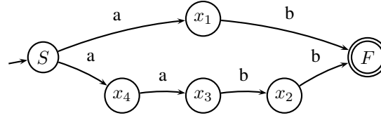
Figure 6. the automaton corresponding to GF(D)
