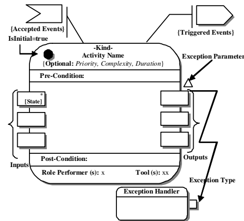
Fig. 2. The UML4SPM Software Activity Notation
