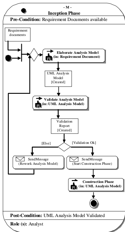
Fig. 2. The UML4SPM Software Activity Notation
