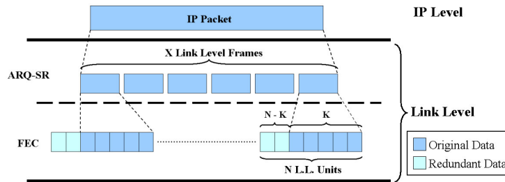
Figure 1: The Hybrid Model FEC / ARQ-SR.
