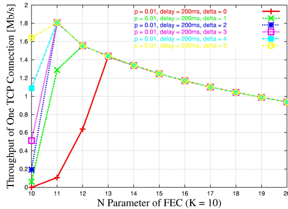
Figure 7 : Throughput of One TCP Connection over the Wireless Link, Hybrid Model.
