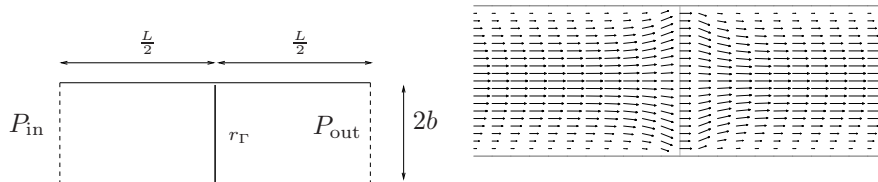
Figure 4: The 2D tube benchmark: straight channel with a straight porous interface. Left: sketch of the domain and boundary conditions. Right: zoom of a numerical solution around the interface ( r_\Gamma = 100 ). For the sake of clarity, we show a relatively coarse mesh.
