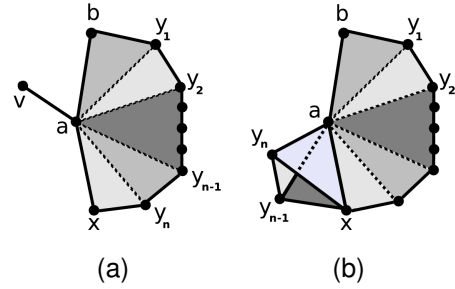
Fig. 18. (a) Ord(\sigma a; \tilde{K}) = 2 since St(a; E) has a half disk and a principal edge. (b) Ord(\sigma a; \tilde{K}) = 2 since ab and ax are incident on one and three triangles respectively.
