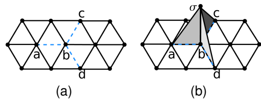
Fig. 5. (a) Simplicial complex K with embedded structure in blue and (b) \tilde{K} obtained by inserting cones from \sigma .
