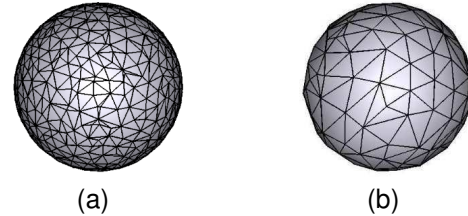
Fig. 2. (a) Embedded structure before and (b) after simplification.
