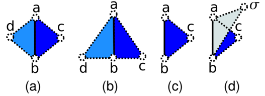
Fig. 9. (a) St(ab; E) contains exactly two triangles abc and abd in the interior of K . (b) Isomorphic subdivision of star of acd . (c) St(ab; E) contains exactly one triangle abc in the interior of K . (d) \sigma ab is incident on one tetrahedron, whereas abc is incident on three tetrahedra.
