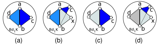
Fig. 8. (a) St(ab; E) contains triangles abc and abd , both lying in Bd_1K . (b) St(ab; E) contains triangle abd on Bd_1K and abc in the interior of K . (c) St(ab; E) contains exactly one triangle abc lying in Bd_1K . (d) St(ab; E) contains exactly one triangle abc lying in the interior of K .
