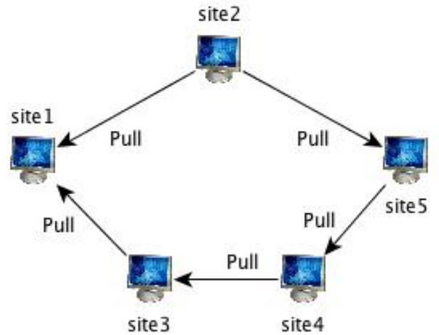
Figure 3: Collaboration scenario
