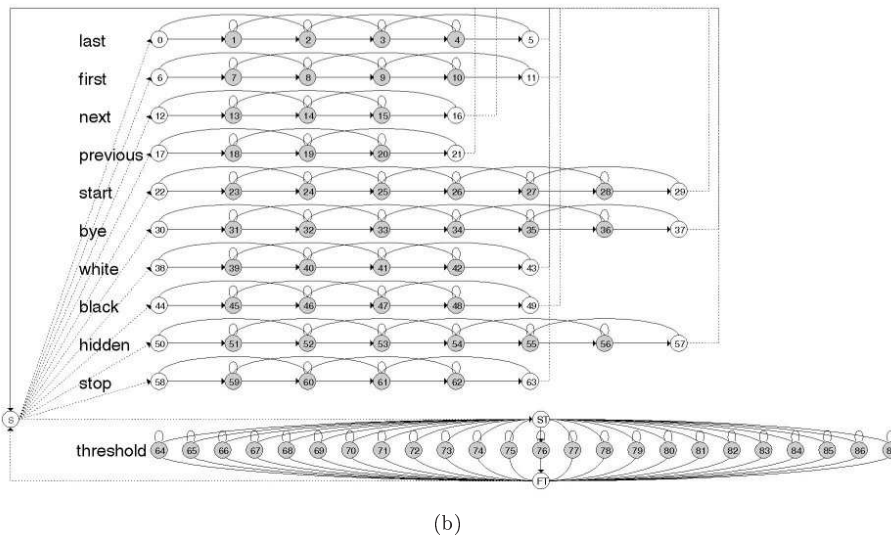
Figure 7: Primitive discovery and garbage modeling using HMMs: (a) Images from [18]. Transition probabilities and initial state probabilities of a fully connected HMM, (Left) before and (Middle) after structure discovery using entropic estimation. (Right) resulting graphical model (b) HMM network with additional garbage-model (threshold model). The garbage model is build as an ergodic fully connected HMM based on copies of all states in the original models from [91]. Awaiting publisher permission
