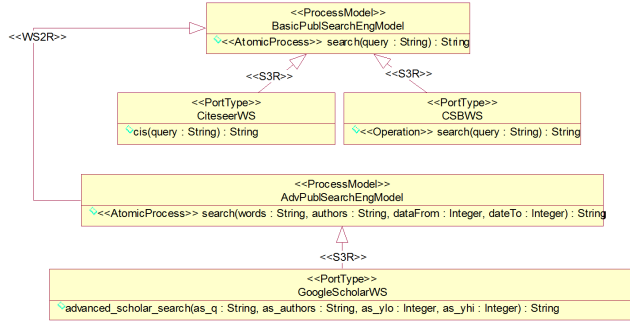
Figure 5: Examples of S3R and WS2R relations.
