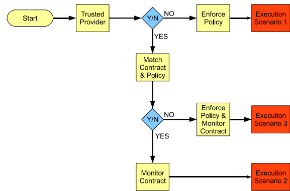
Figure 2: The Extended Security-by-Contract Application life-cycle.
