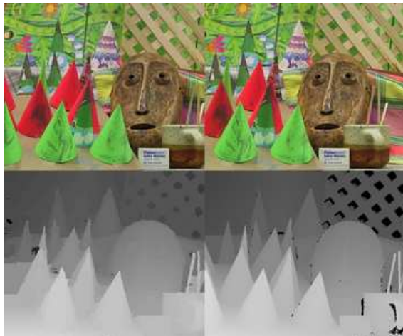
Fig. 29. Disparities for Cones - 104.2s. - 89.09%
