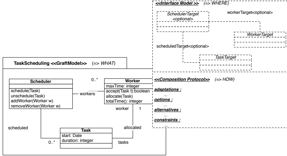
Fig. 1. The task allocation aspect
