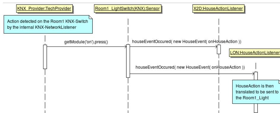
Fig. 3. Message transmission on action detection
