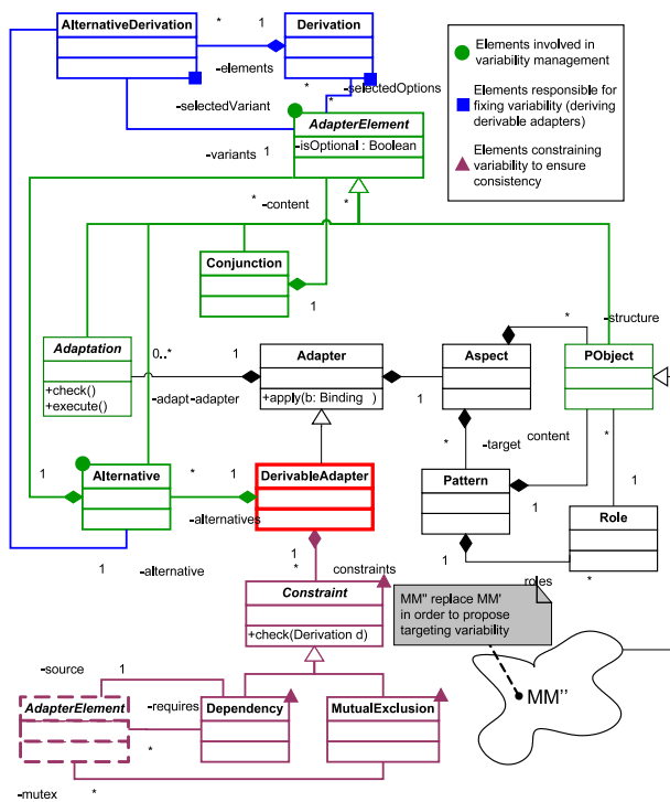
Figure 5. Extended Adaptation Metamodel
