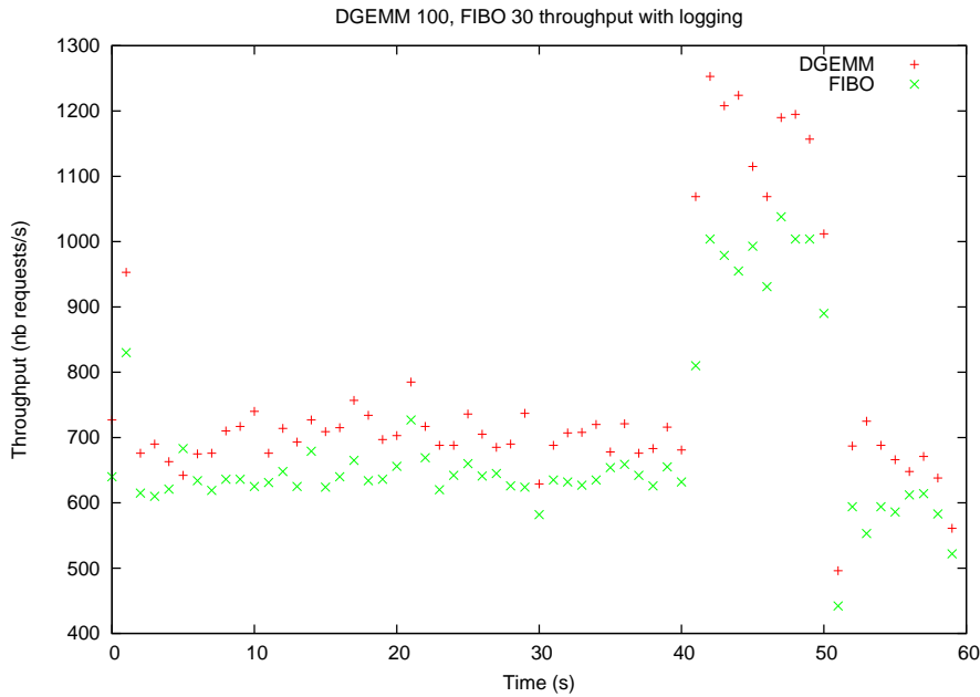
Figure 49: Throughput for dgemm 100, Fibonacci 30. With logging on.
