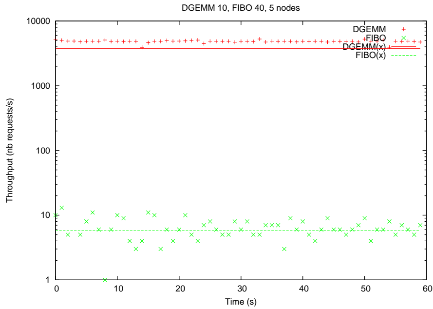
Figure 27: Throughputs for services dgemm 10 and Fibonacci 40, on 5 nodes.
