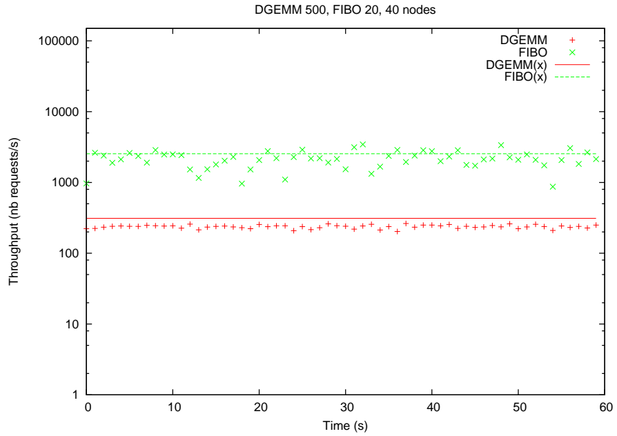
Figure 38: Throughputs for services dgemm 500 and Fibonacci 20, on 40 nodes.
