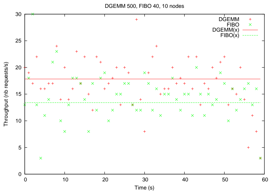
Figure 42: Throughputs for services dgemm 500 and Fibonacci 40, on 10 nodes.
