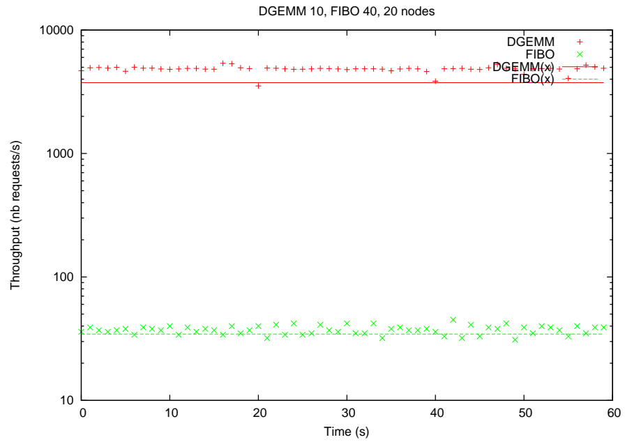
Figure 29: Throughputs for services dgemm 10 and Fibonacci 40, on 20 nodes.
