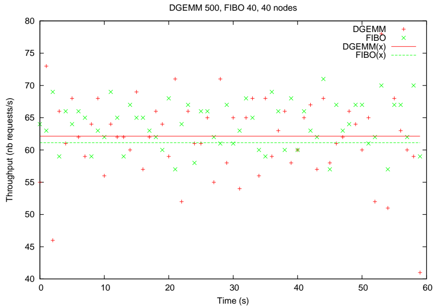
Figure 45: Throughputs for services dgemm 500 and Fibonacci 40, on 40 nodes.
