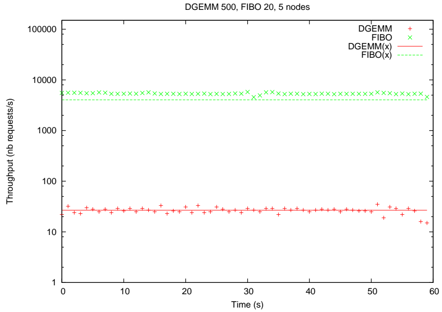
Figure 34: Throughputs for services dgemm 500 and Fibonacci 20, on 5 nodes.
