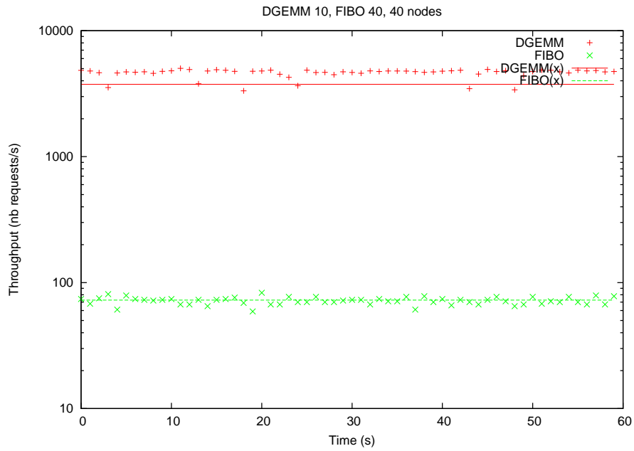
Figure 31: Throughputs for services dgemm 10 and Fibonacci 40, on 40 nodes.
