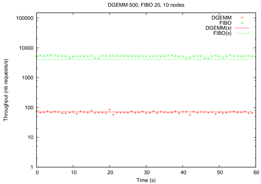
Figure 35: Throughputs for services dgemm 500 and Fibonacci 20, on 10 nodes.
