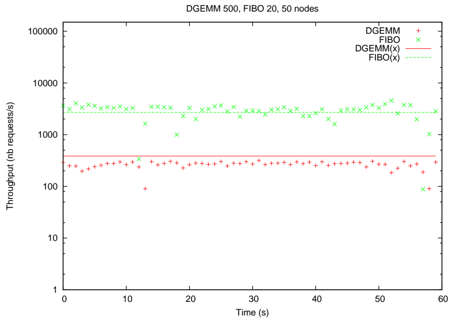
Figure 39: Throughputs for services dgemm 500 and Fibonacci 20, on 50 nodes.
