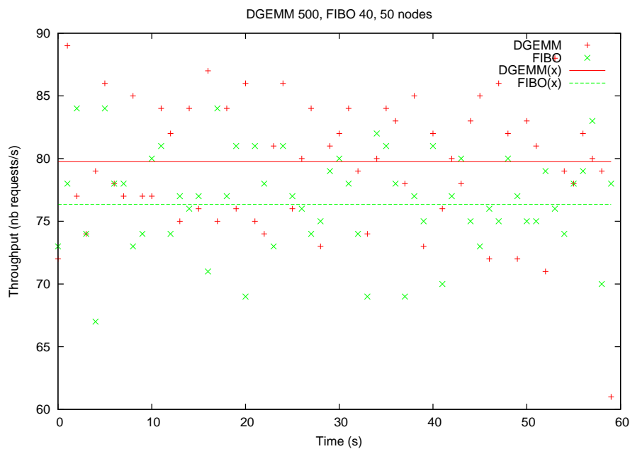
Figure 46: Throughputs for services dgemm 500 and Fibonacci 40, on 50 nodes.
