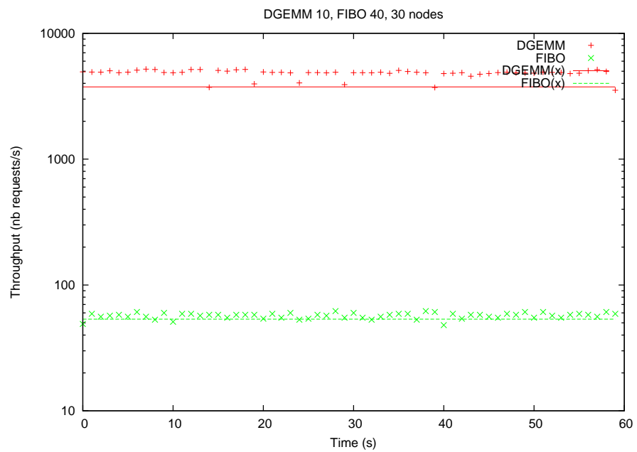
Figure 30: Throughputs for services dgemm 10 and Fibonacci 40, on 30 nodes.
