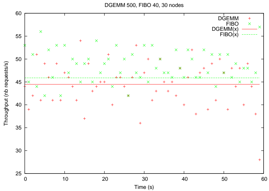
Figure 44: Throughputs for services dgemm 500 and Fibonacci 40, on 30 nodes.
