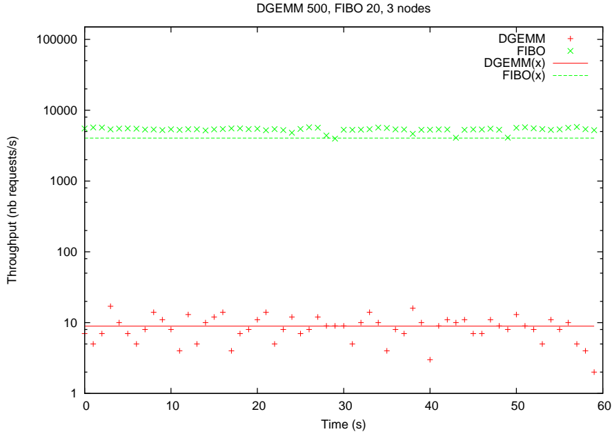
Figure 33: Throughputs for services dgemm 500 and Fibonacci 20, on 3 nodes.
