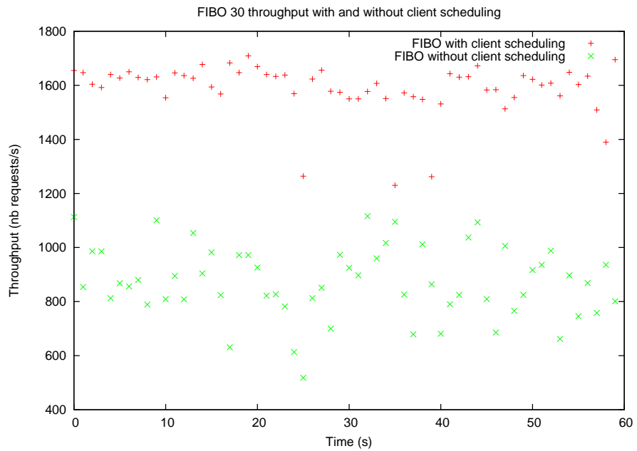
Figure 48: Throughput for Fibonacci 30 with and without client scheduling.
