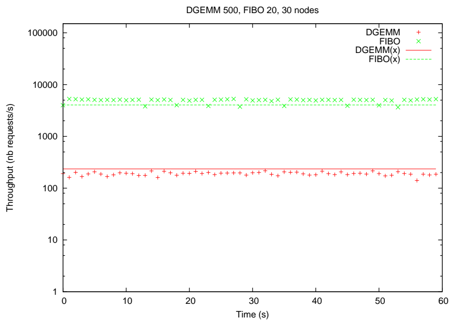
Figure 37: Throughputs for services dgemm 500 and Fibonacci 20, on 30 nodes.
