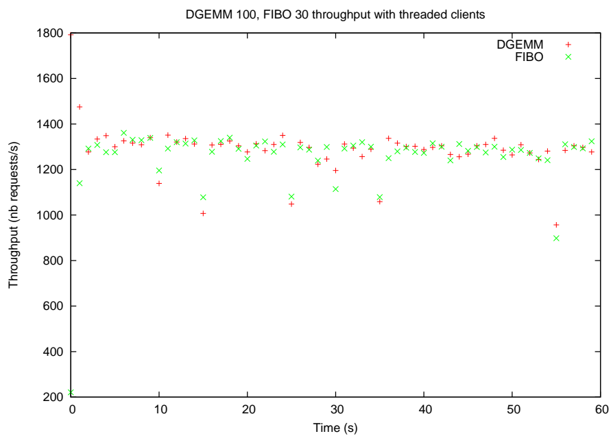
Figure 52: Throughput for dgemm 100, Fibonacci 30. 10 dgemm threaded clients (15 threads each), and 2 Fibonacci threaded clients (75 threads each). Each client is on a separate node.
