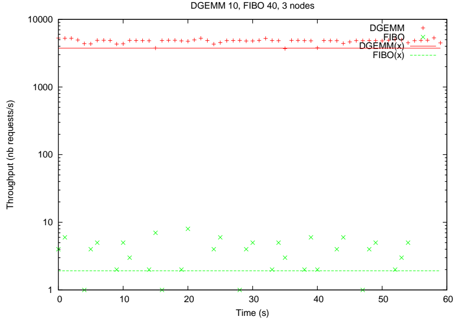
Figure 26: Throughputs for services dgemm 10 and Fibonacci 40 , on 3 nodes.
