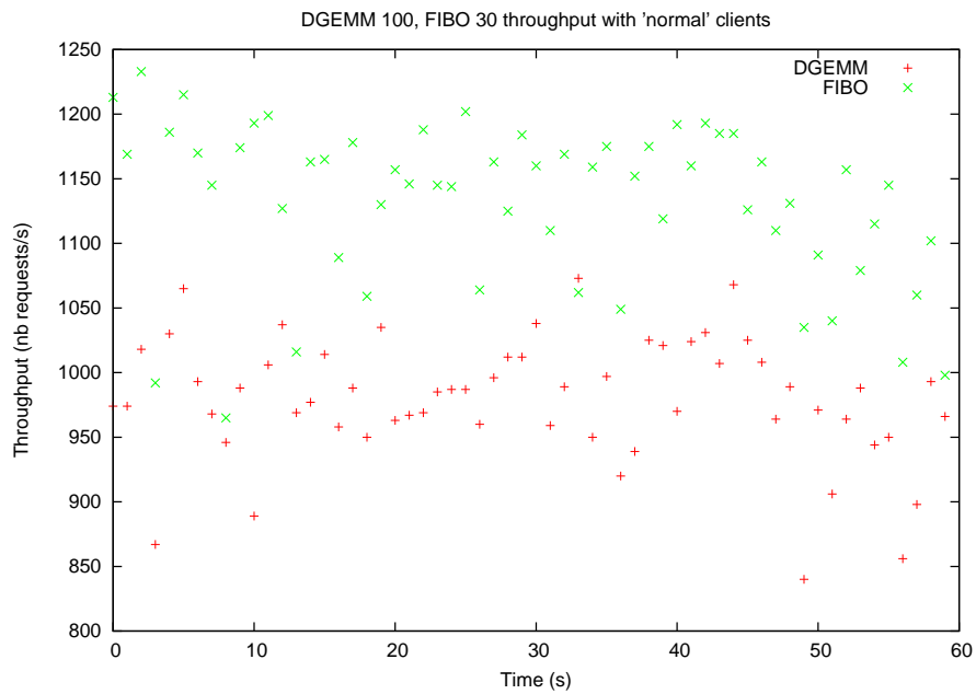
Figure 51: Throughput for dgemm 100, Fibonacci 30. 150 dgemm and FIBO “normal” clients on 40 different nodes.
