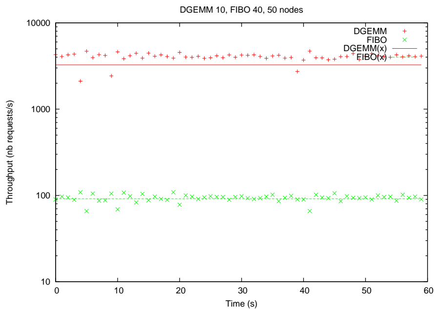
Figure 32: Throughputs for services dgemm 10 and Fibonacci 40, on 50 nodes.
