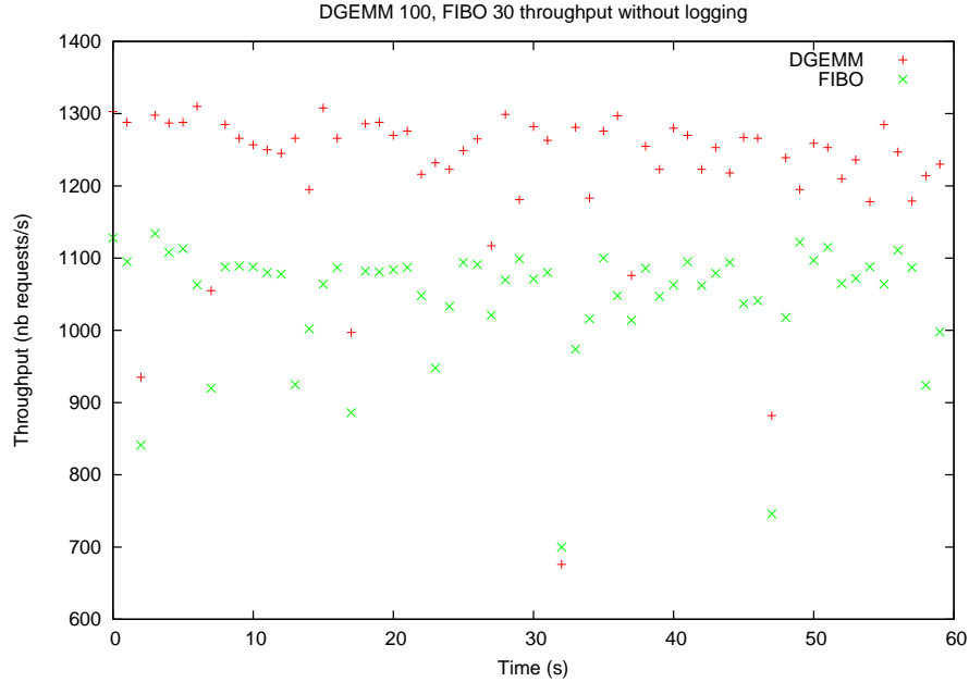
Figure 50: Throughput for dgemm 100 , Fibonacci 30. With logging off.
