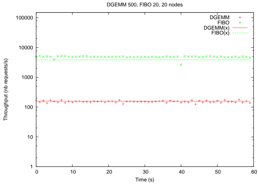
Figure 36: Throughputs for services dgemm 500 and Fibonacci 20, on 20 nodes.
