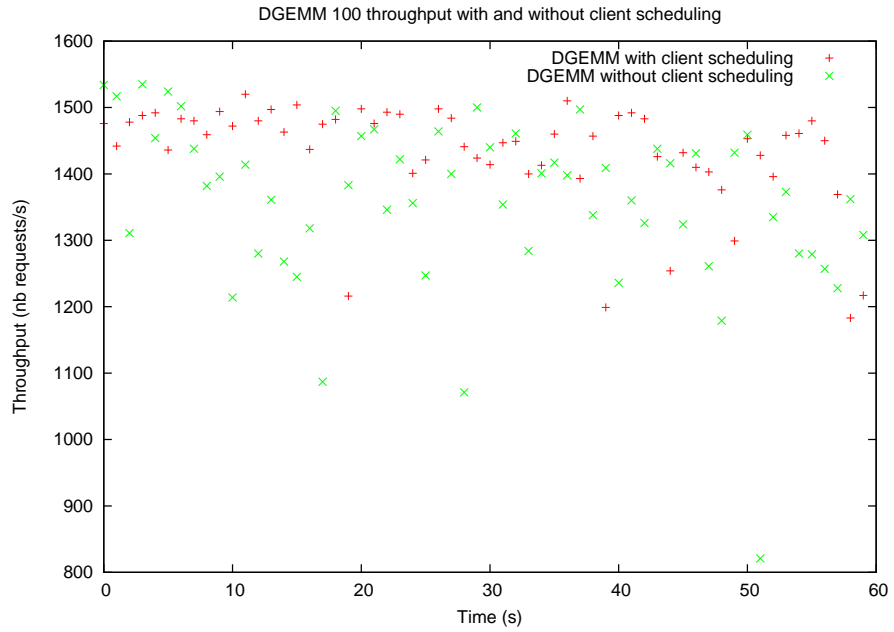
Figure 47: Throughput for dgemm 100 with and without client scheduling.
