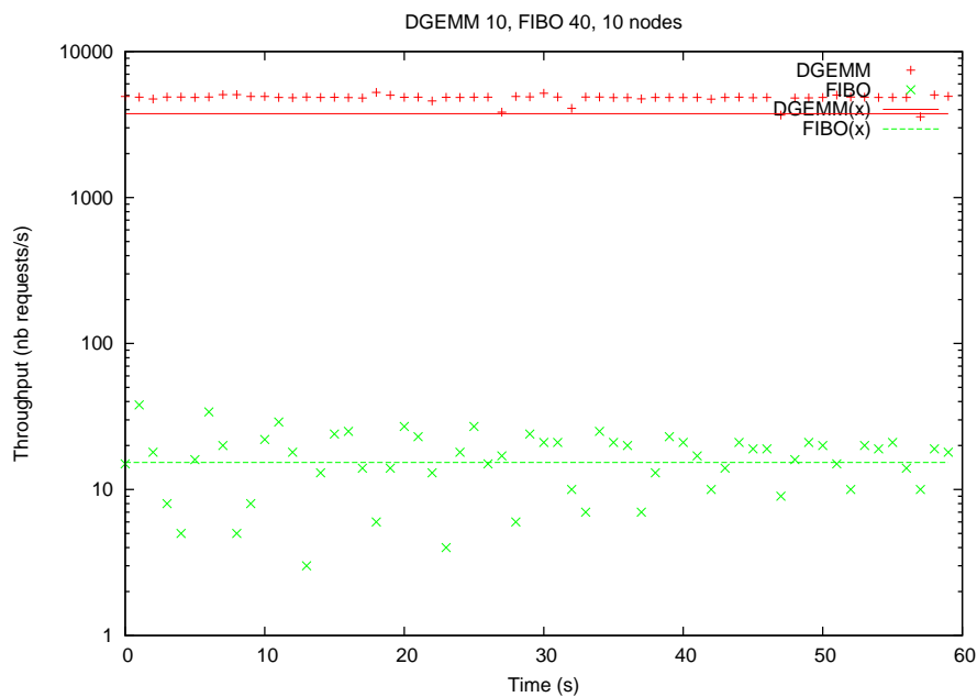
Figure 28: Throughputs for services dgemm 10 and Fibonacci 40, on 10 nodes.
