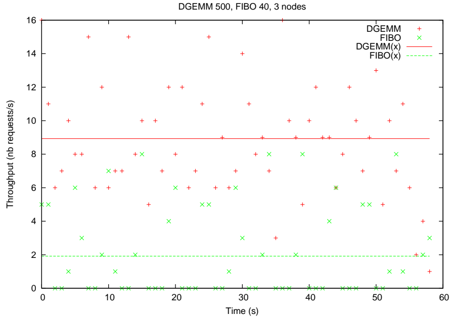
Figure 40: Throughputs for services dgemm 500 and Fibonacci 40 , on 3 nodes.
