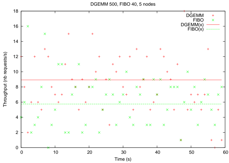
Figure 41: Throughputs for services dgemm 500 and Fibonacci 40, on 5 nodes.
