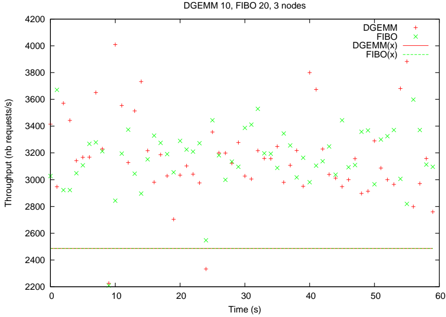
Figure 25: Throughputs for services dgemm 10 and Fibonacci 20 , on 3 nodes.
