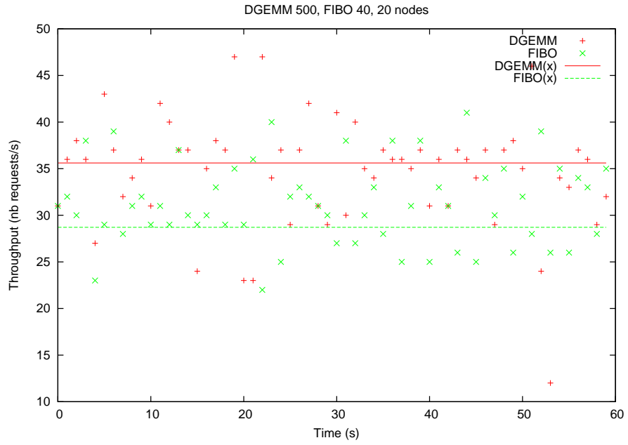
Figure 43: Throughputs for services dgemm 500 and Fibonacci 40, on 20 nodes.
