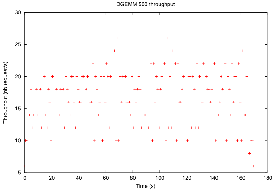
Figure 15: dgemm 500 throughput
