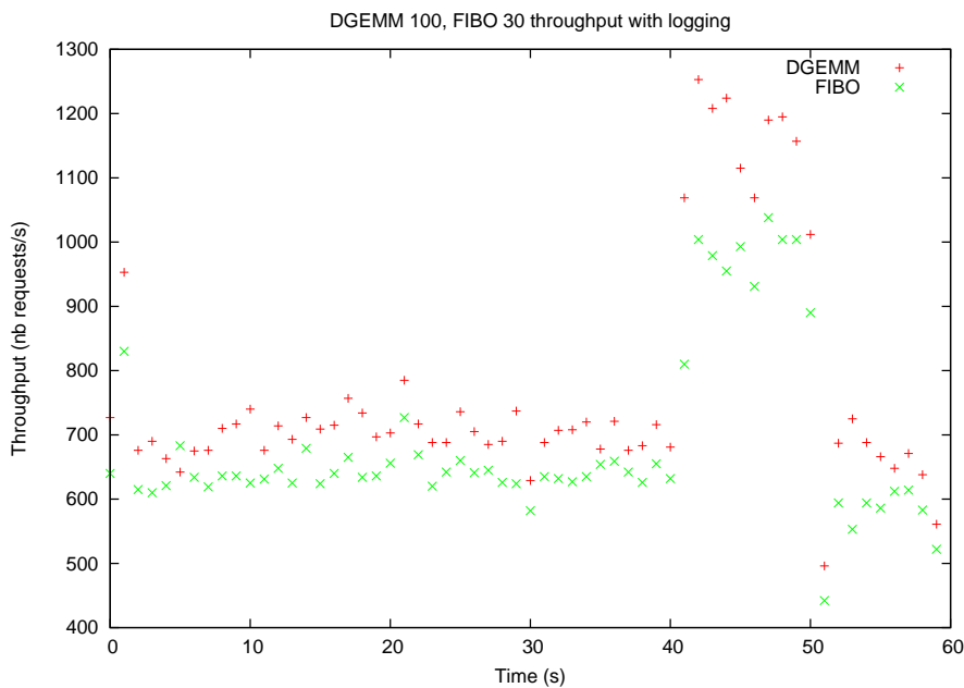
Figure 49: Throughput for dgemm 100, Fibonacci 30. With logging on.
