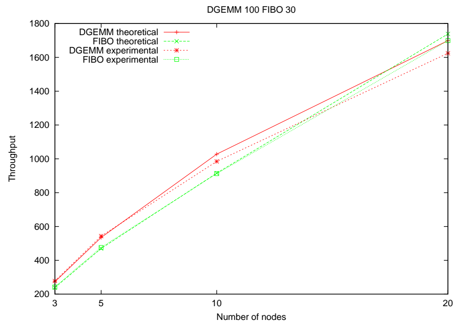
Figure 25: Comparison theoretical/experimental results, for dgemm 100 Fibonacci 30.
