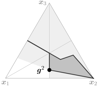
Figure 3: Extremality of \mathbf{g}^2
