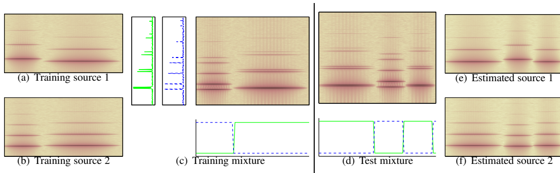
Figure 1: in a simple case, 2 sources (spectrograms (a) and (b)) are mixed to train a 2-joint-state model ((c), with learned DSPs vertically on the left and related posteriors horizontally down below). A test signal (d) is separated (estimated posterior down below) into (e) and (f).
