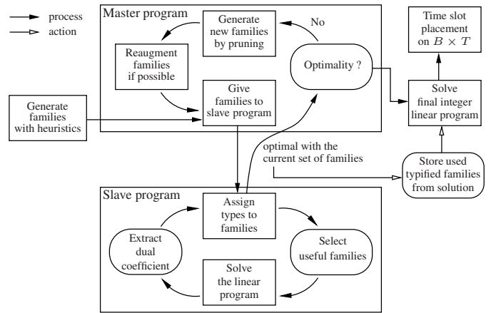
Figure 10: Algorithm overview.
