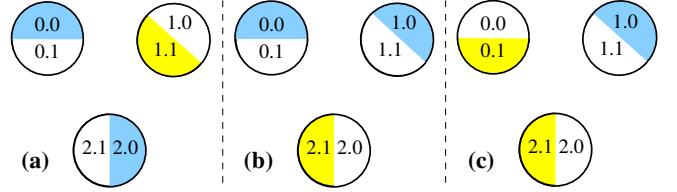
Figure 4: Valid 3-spot combinations for a threshold \sigma = 0.30 .
