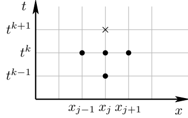
Figure 1: Three-point scheme: u_j^{k+1} (×) depends on u_{j-1}^k , u_j^k , u_{j+1}^k and u_j^{k-1} (•).
