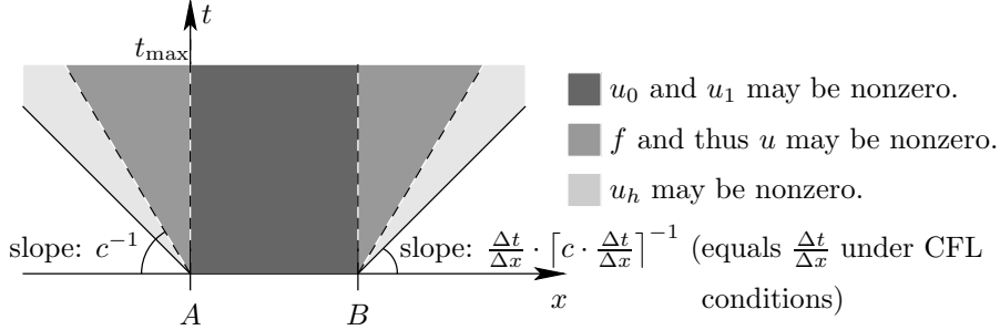
Figure 2: Finite supports. The support of the Cauchy data u_0 and u_1 is included in the support of the continuous source term f , and of the continuous solution u . Which is in turn also included in the support of the discrete solution u_h , provided that the CFL condition holds. For a finite t_{\max} , all these supports are finite.
