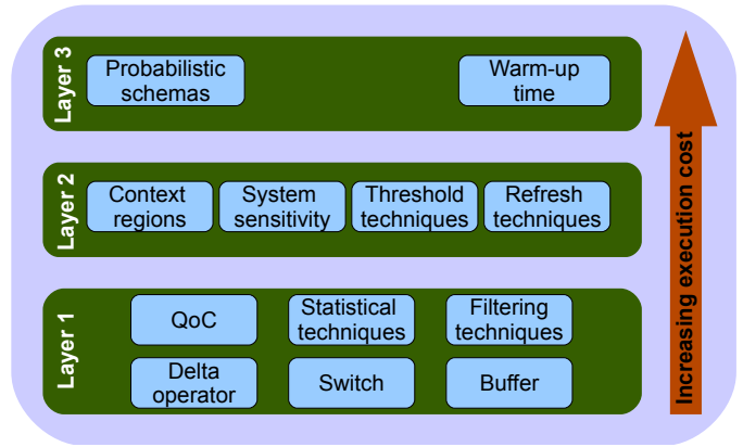
Fig. 1. Conceptual architecture
