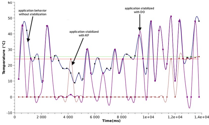
Fig. 7. Stabilized application behavior - Kalman filter and Delta operator
