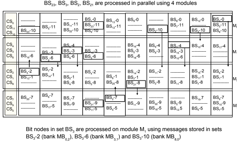
Figure 5. Data memory organization and scenario example for bit node and check node processing.
