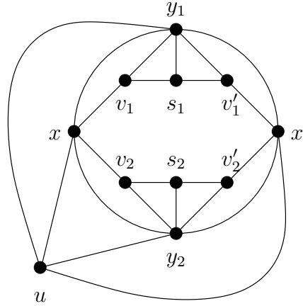
Figure 7: A graph G \in CW(2) which is not strongly 2-bidismantlable.
