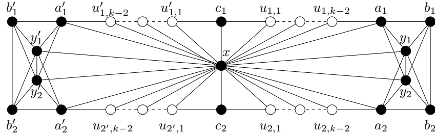
Figure 7: A graph G \in CWW(k) that is not k -bidismantlable
