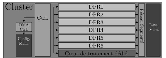
Figure 10. Resource allocation of the implemented DPR of DART
