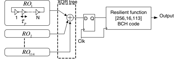
Fig. 3. Oscillator sampling proposed by Sunter et al [6].
