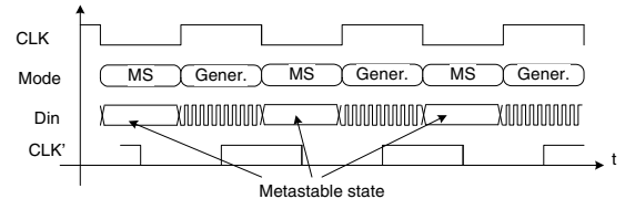
Fig. 5. TRNG generation by using the META-RO circuit.
