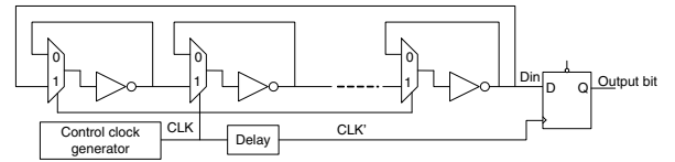
Fig. 4. META-RO architecture proposed by Vasylytsov and al [7].
