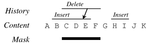
Figure 7 Babble represents a text buffer in three layers. This buffer is displayed as ABGHIJK
