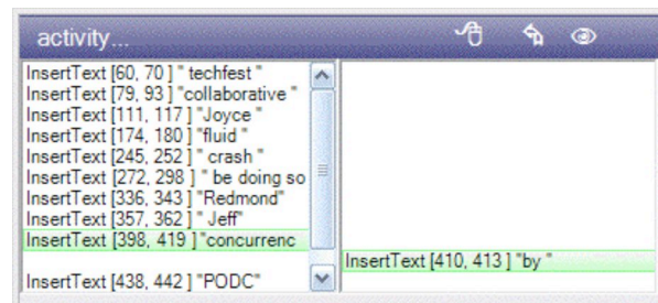
Figure 12 The history editor
