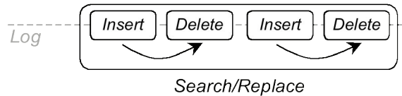
Figure 1 Joyce logs modifications with their semantics. A text editor may model search and replace as insert and delete actions that are ordered and atomic.
