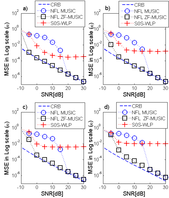
Figure 5: MSE( \omega rad) vs. SNR[dB], Largely spaced sources ( \omega_1 = 0.5 , \phi_1 = 0.015 ) rad and ( \omega_2 = 1.2 , \phi_2 = 0.06 ) rad, with 12 sensors and 15 snapshots; (a) \gamma = 0 , (b) \gamma = 0.3 , (c) \gamma = 0.5 , (d) \gamma = 0.8 .
