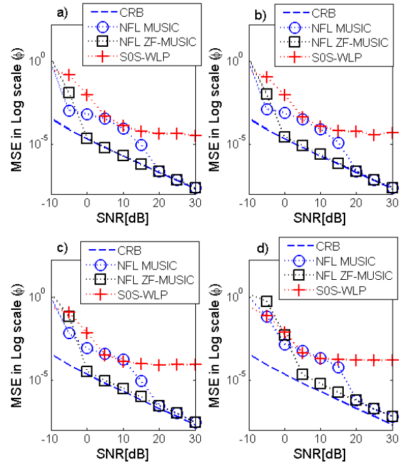
Figure 6: MSE( \phi rad) vs. SNR[dB], Largely spaced sources ( \omega_1 = 0.5 , \phi_1 = 0.015 ) rad and ( \omega_2 = 1.2 , \phi_2 = 0.06 ) rad, with 12 sensors and 15 snapshots; (a) \gamma = 0 , (b) \gamma = 0.3 , (c) \gamma = 0.5 , (d) \gamma = 0.8 .
