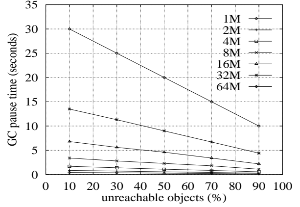
Figure 4. Non-concurrent mark-and-sweep.
