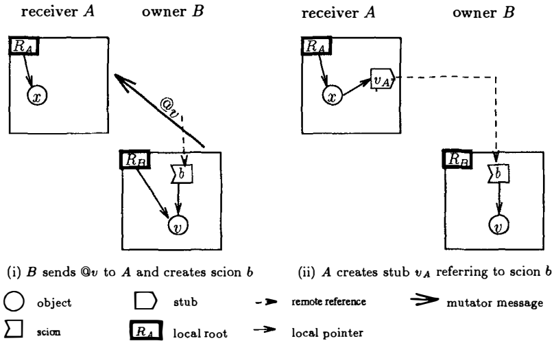
Figure 1: Remote reference creation.
