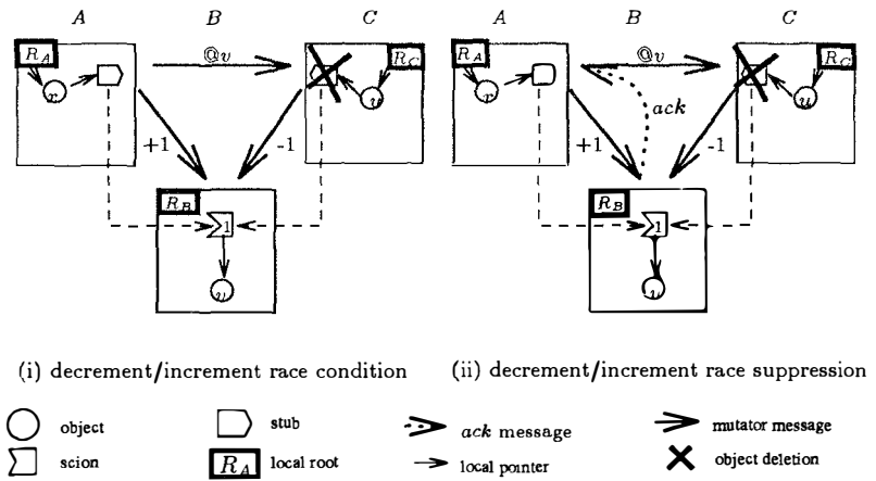
Figure 5: Race conditions between increment and decrement messages.
