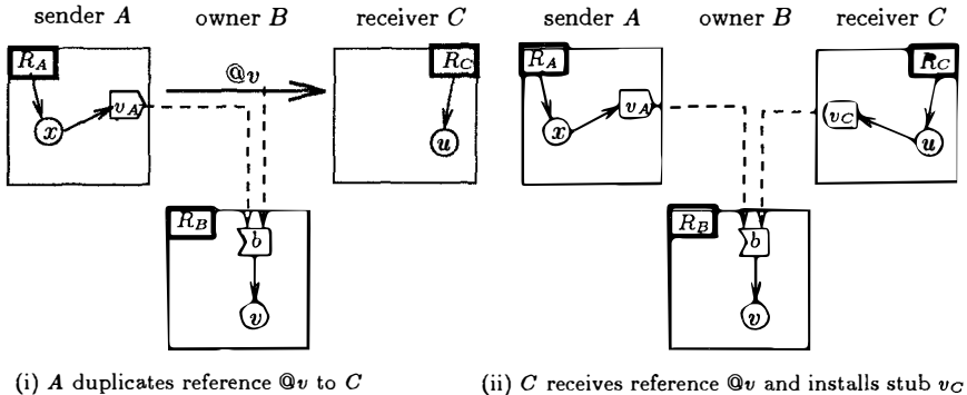
Figure 2: Remote reference duplication.
