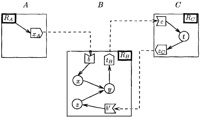
Figure 16: Rudalics’ counter-example to Liskov’s central service.
