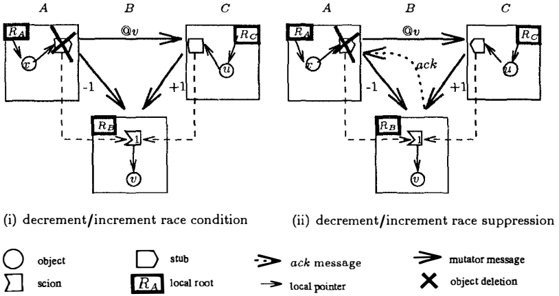
Figure 4: Race conditions between decrement and increment messages.
