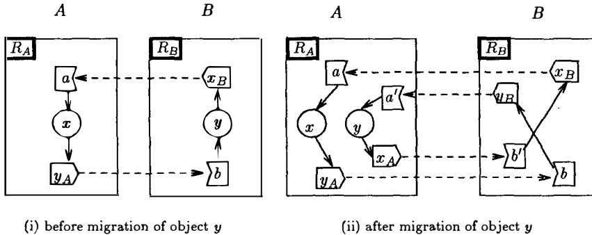
Figure 11: Bishop's migration techniques conflicts with indirections.
