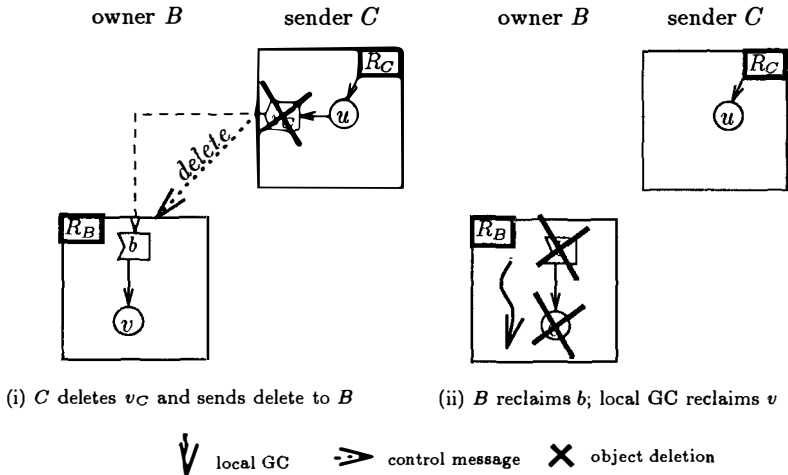
Figure 3: Remote reference deletion.
