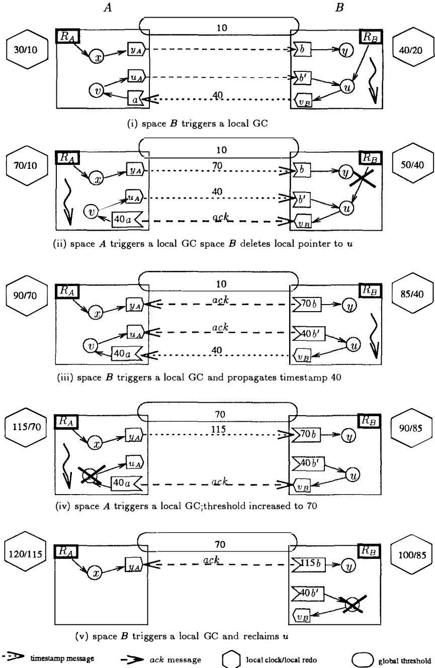
Figure 15: Example of Hughes' timestamping technique.
