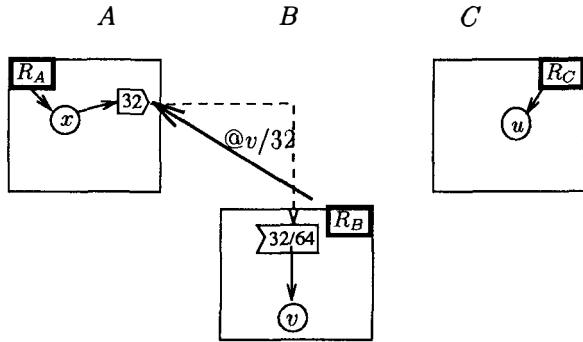
(i) B creates a reference to v with a partial weight equal to 32
