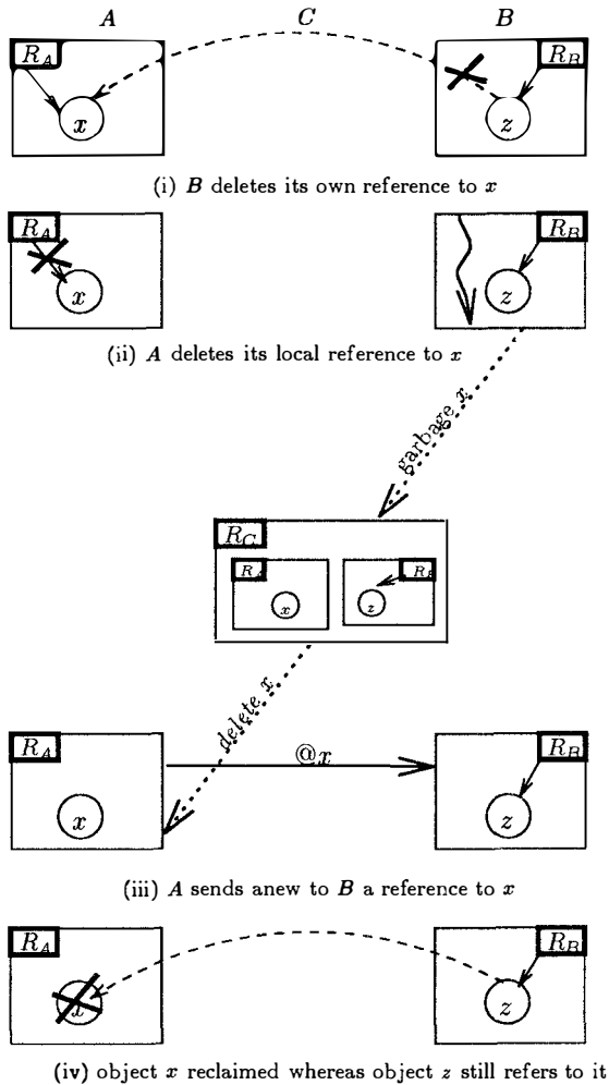
Figure 14: Message in transit problem.
