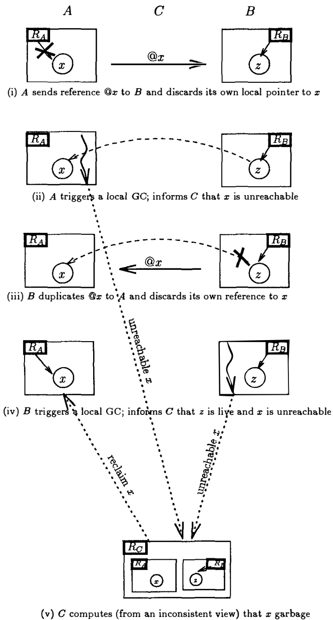
Figure 13: Inconsistent GC snapshot.
