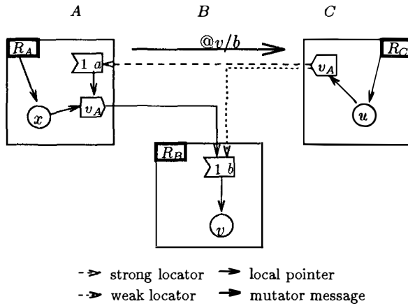
Figure 8: Reference duplication in Indirect Reference Counting.
