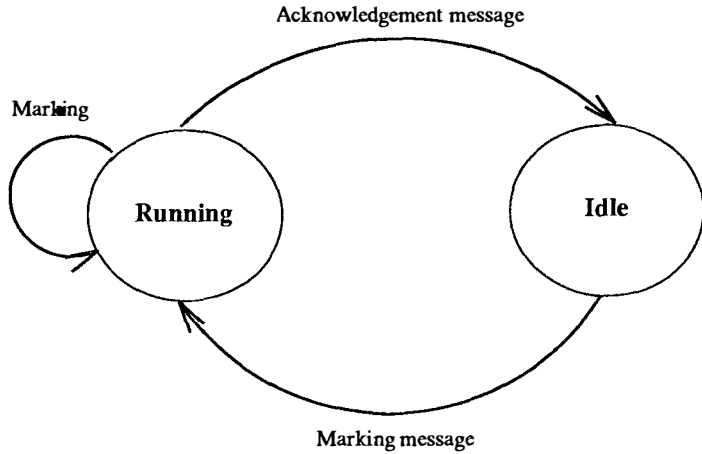
Figure 12: Distributed tracing.
