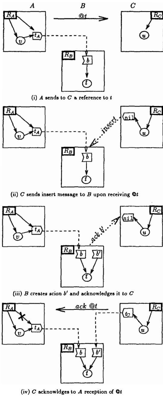
Figure 9: Duplication of a reference to a network object.
