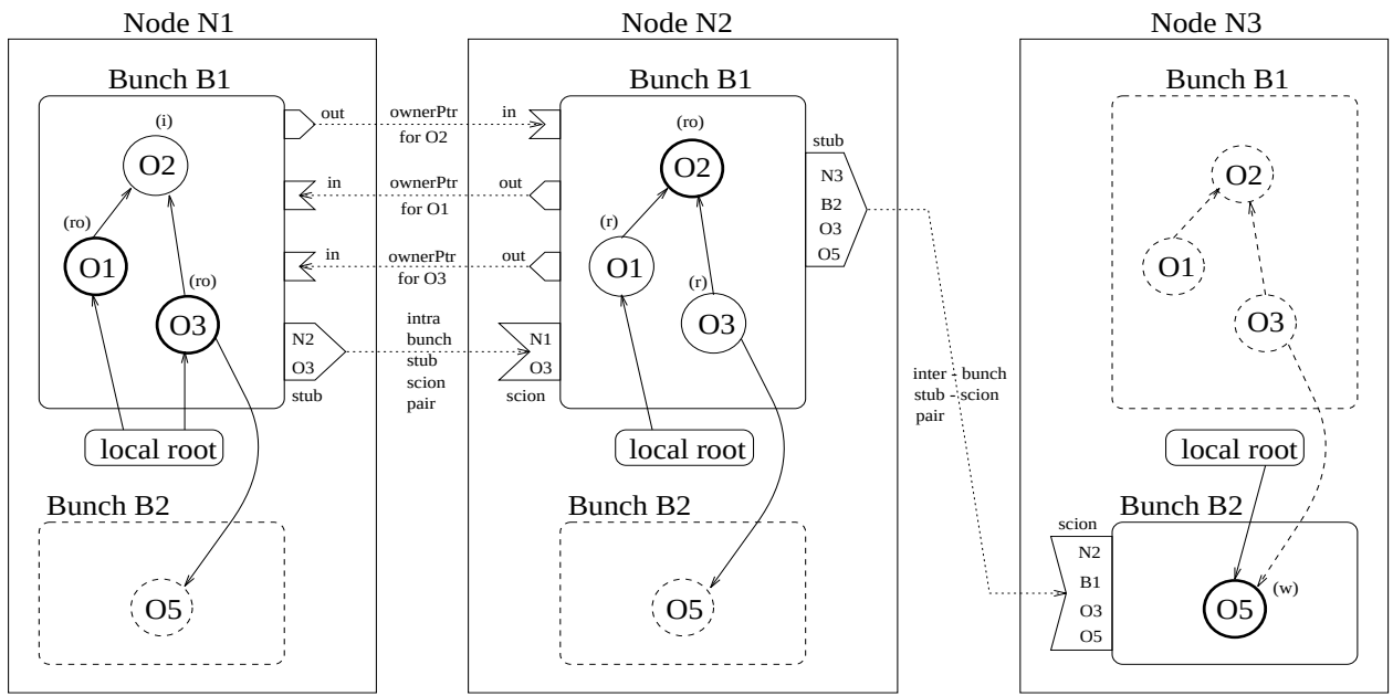
Figure 1: Bunch B1 is mapped on nodes N1 and N2 , and bunch B2 is mapped only on N3 ; mapped bunches are represented with a solid line, unmapped bunches are represented with a dashed line. Stub and scion tables contain inter-bunch and intra-bunch SSPs. For each object, the state of its token is indicated as follows: letters r and w indicate that the node has a read or a write token respectively; o means that the node is the object’s owner (thicker objects); i is used for inconsistent copies. The local root includes mutator stacks. No GC has taken place on any node.
