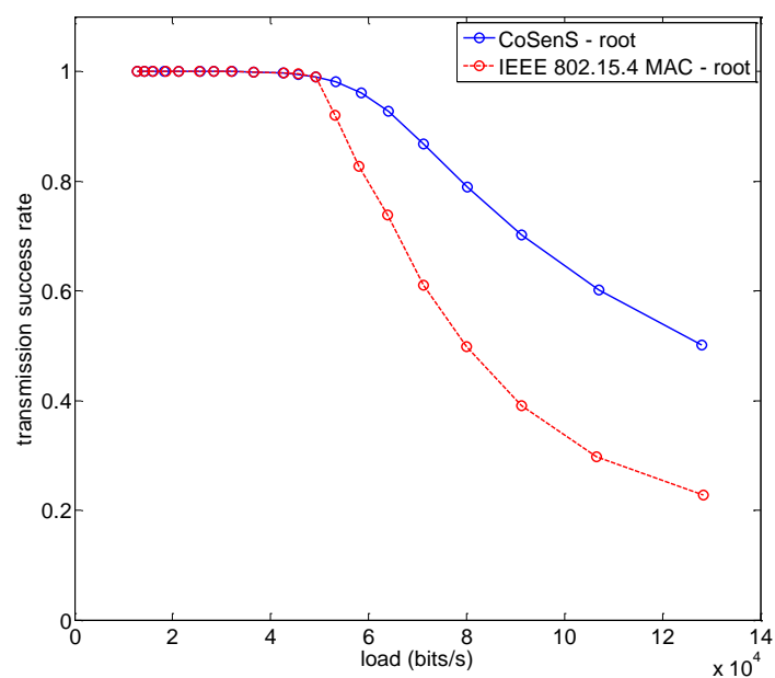
Fig. 36. Transmission success probability of scenario 8.
