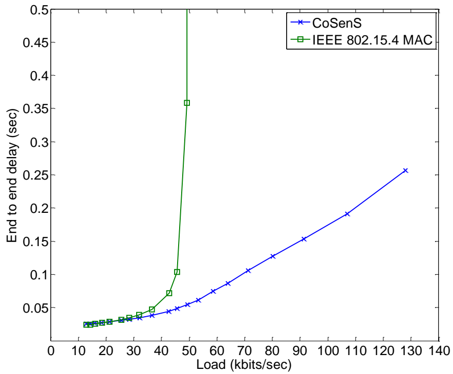
Fig. 37. End-to-end delay of scenario 8.
