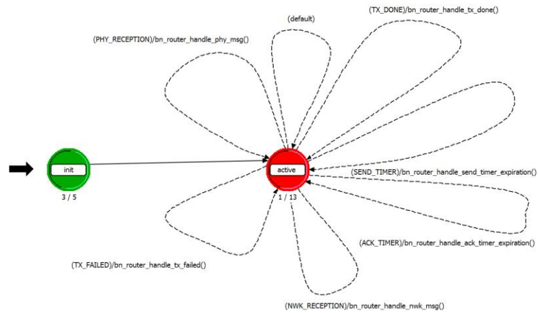
Fig. 4. MAC process model
