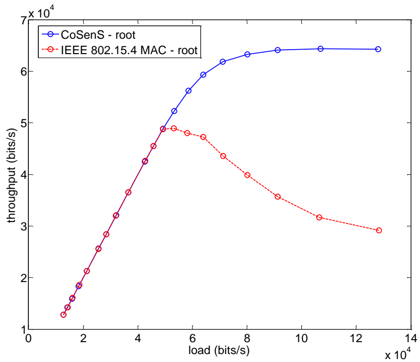
Fig. 38. Throughput of scenario 8.
