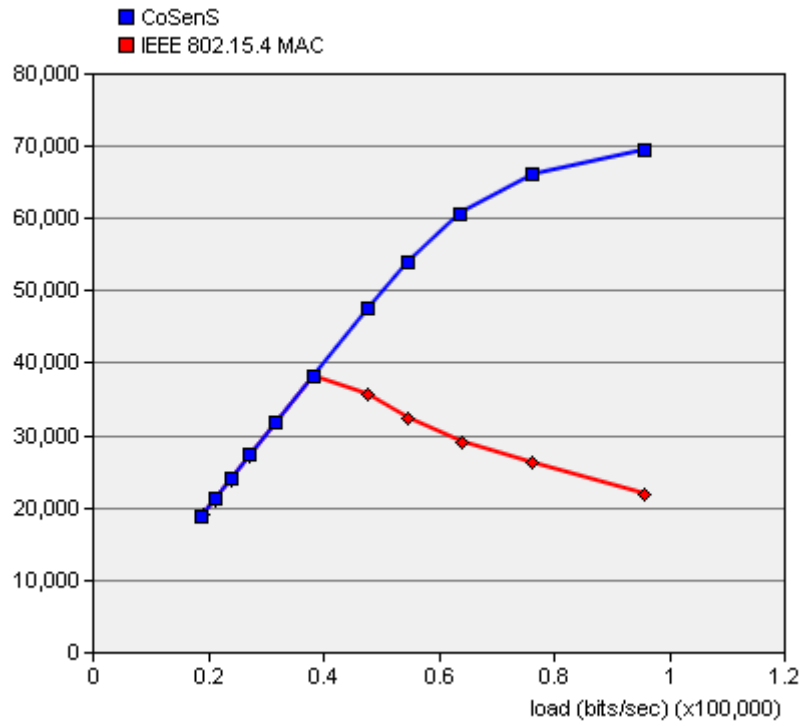
Fig. 19. Throughput (bits/sec) for scenario 3.
