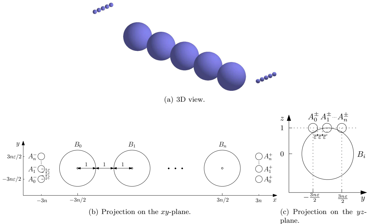
Figure 1: Illustration of our construction for Theorem 1.
