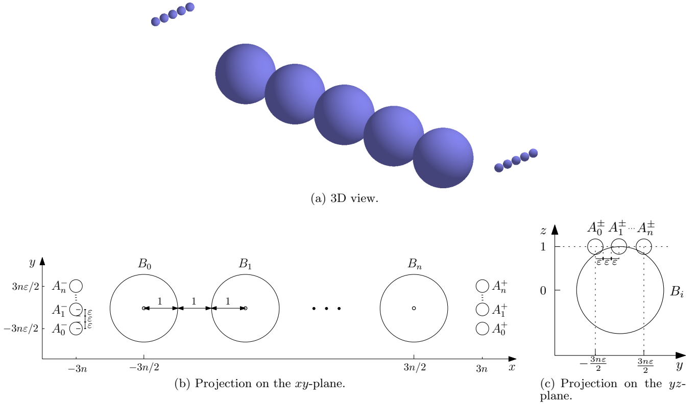
Figure 1: Illustration of our construction for Theorem 1.
