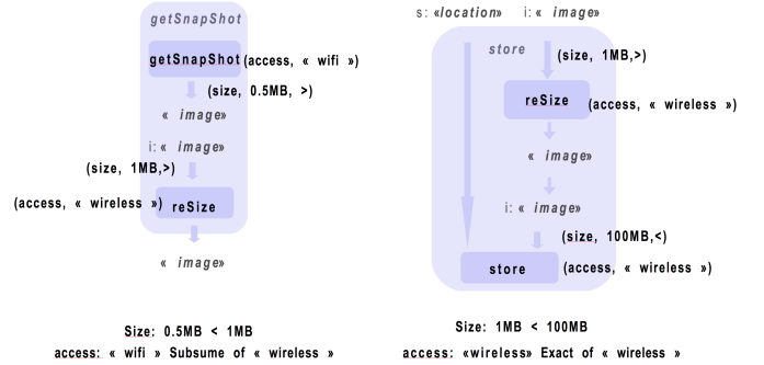
Figure 6. User-centric operation composition
