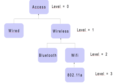
Figure 3. access ontology
