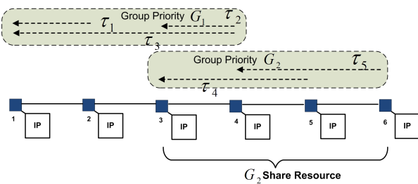
Figure 2. A Case of Traffic-flows with Priority Share
