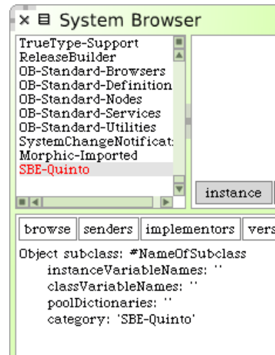
Figure 2.3: The class-creation Template.
