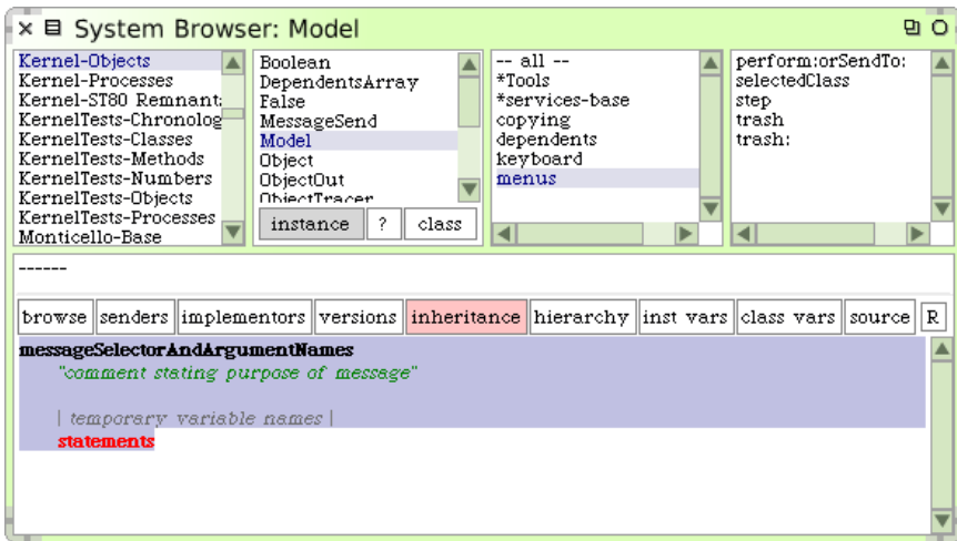
Figure 6.5: System Browser showing the method-creation template
