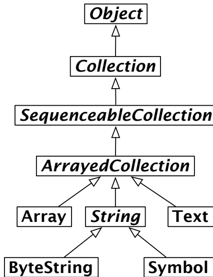
Figure 8.2: The String Hierarchy
