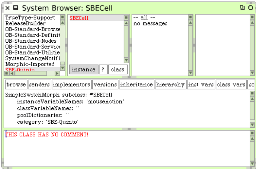
Figure 2.5: The newly-created class SBECell
