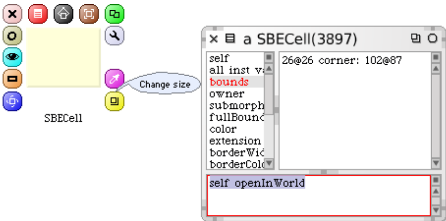
Figure 2.7: Resizing the cell.
