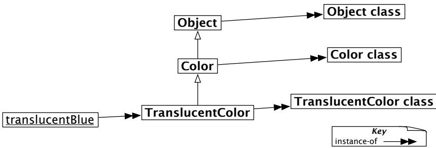
Figure 12.3: The metaclasses of Translucent and its superclasses
