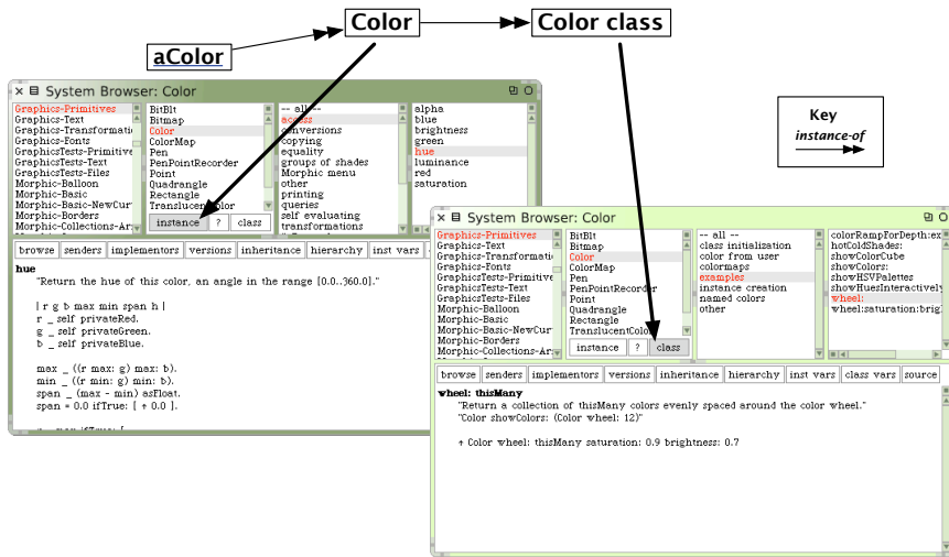
Figure 5.1: Browsing a class and its metaclass.
