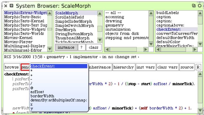
Figure 6.6: A Class Browser opened on the ScaleMorph class. Note the horizontal bar of buttons at the center of the browser; here we are using the senders button.
