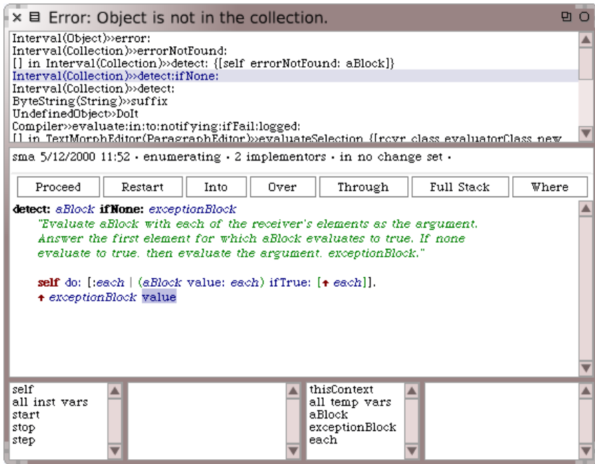
Figure 6.25: The debugger.
