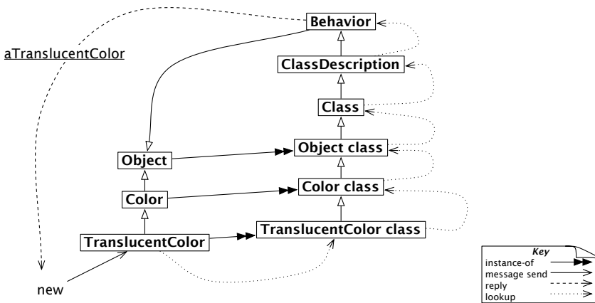
Figure 12.8: new is an ordinary message looked up in the metaclass chain.
