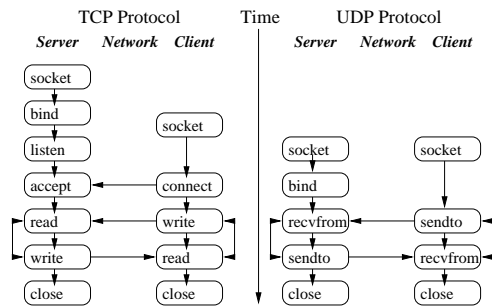
Figure 1: Typical usage of the TCP and UDP APIs.
