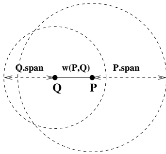
Figure 2: Invariant LI(iv) .
